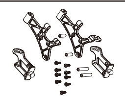
BS809-011 Wing mount (Lf/Rt) Bushing & screws
