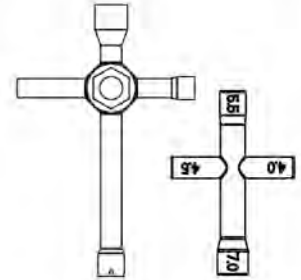
Large & small cross-wrenches
