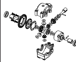
BS803-025 Diff. gearbox unit
