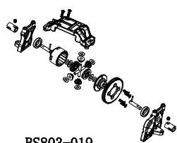
BS803-019 Centre diff. Unit
