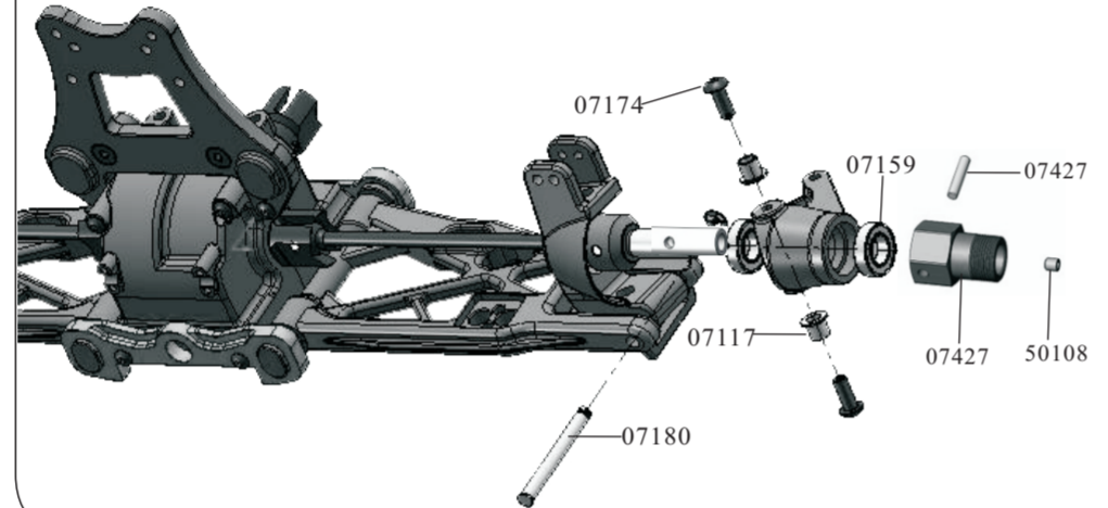
Steering Mount Assembly
