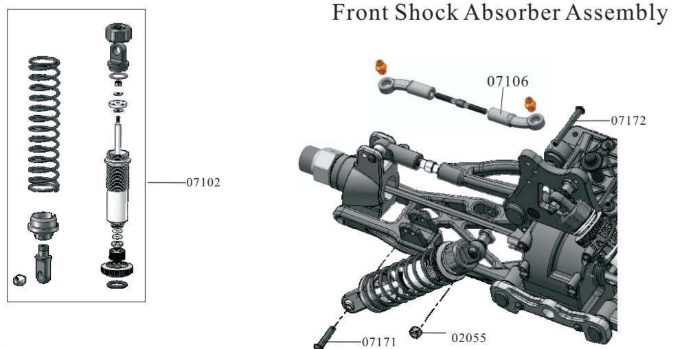
Front Shock Absorber Exploded View(Short)
