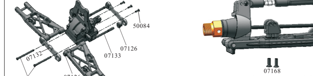
Front lower Suspension Arms Assembly
