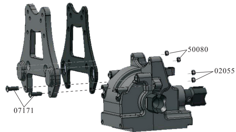
Rear Shock Tower Assembly
