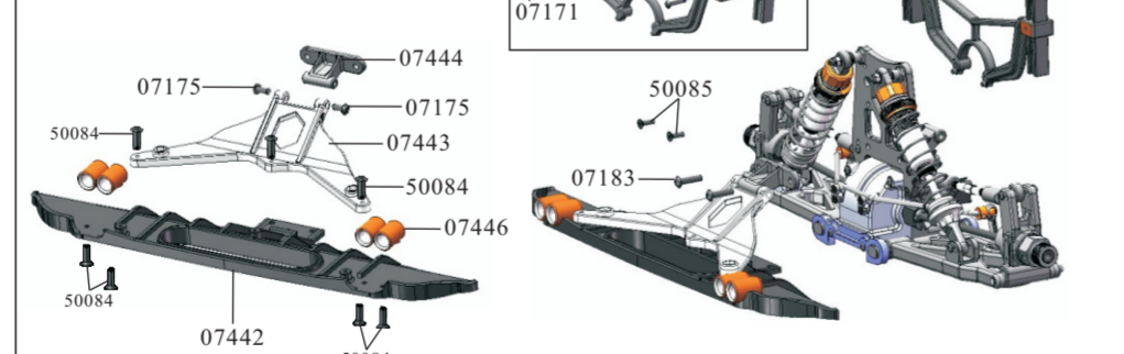
Rear body post Assembly
