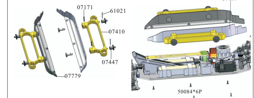
Side Guard Assembly(R/L)
