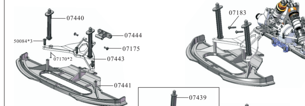
Front body post Assembly
