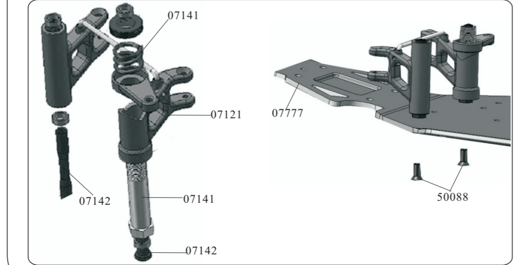
Front Shock Absorber Assembly
