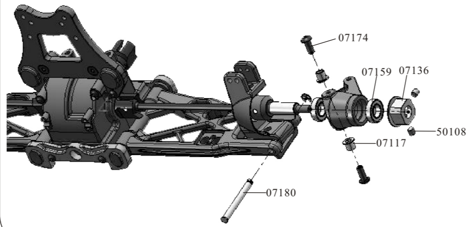
Steering Mount Assembly
