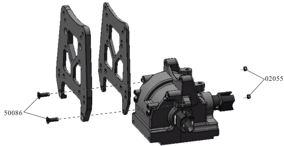
Rear Shock Tower Assembly
