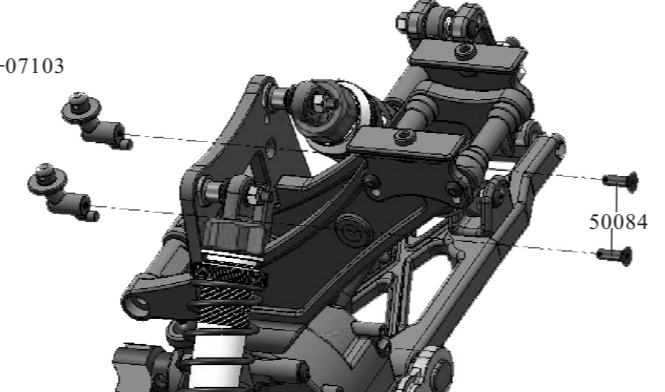
Rear body post Assembly
