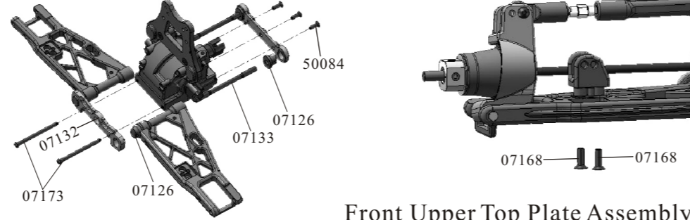
Front Upper Suspension Arms Assembly
