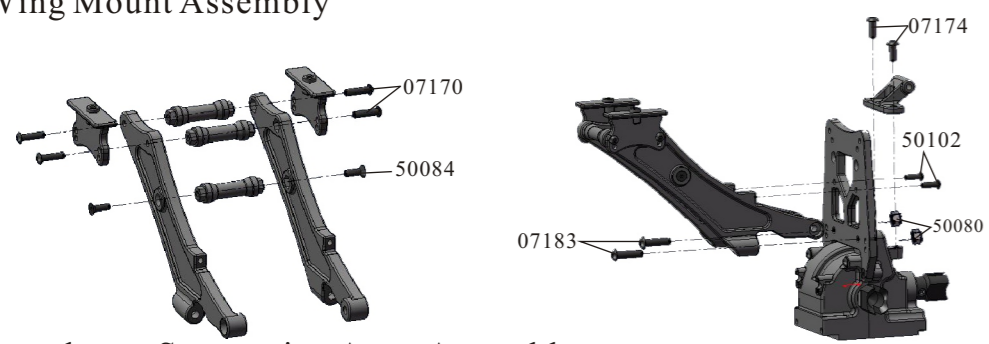
Rear lower Suspension Arms Assembly
