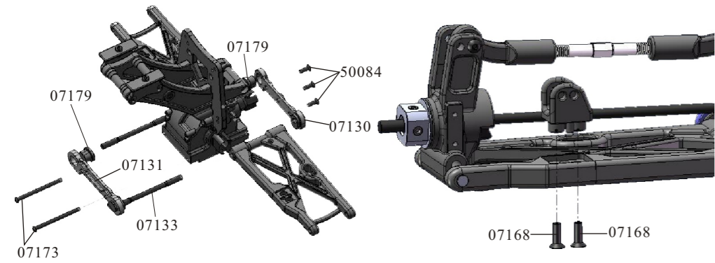
Rear Upper Suspension Arms Assembly
