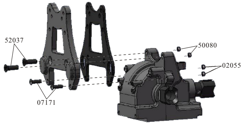
Rear Shock Tower Assembly
