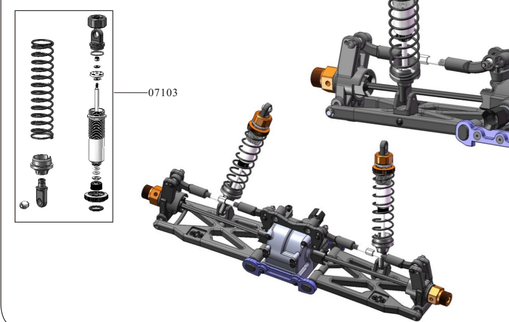
Rear Shock Absorber Exploded View(long)
