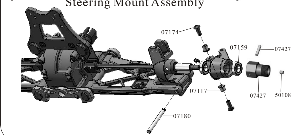
Steering Mount Assembly
